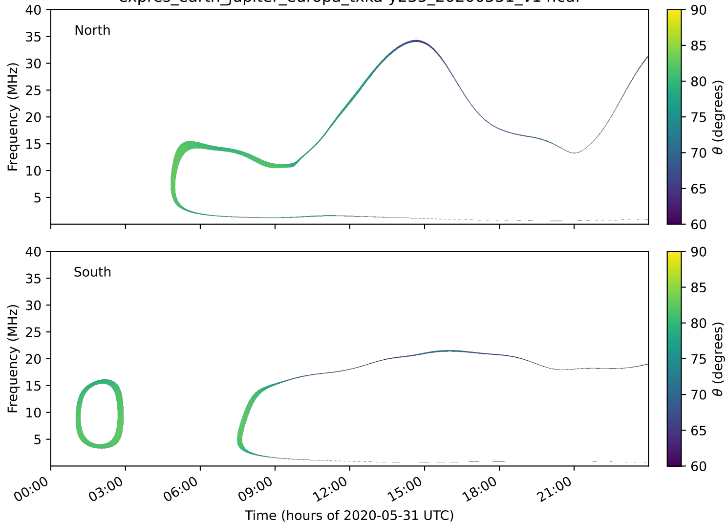
expres_earth_jupiter_europa_txka-y235_20200531_v14.cdf
