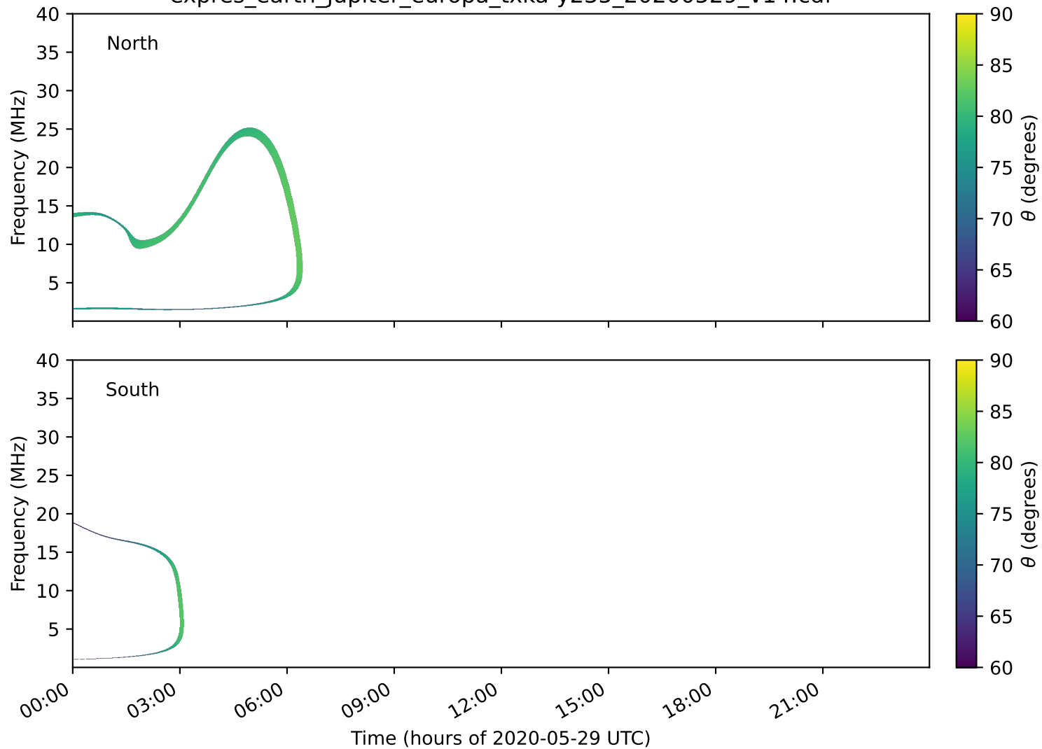
expres_earth_jupiter_europa_txka-y235_20200529_v14.cdf
