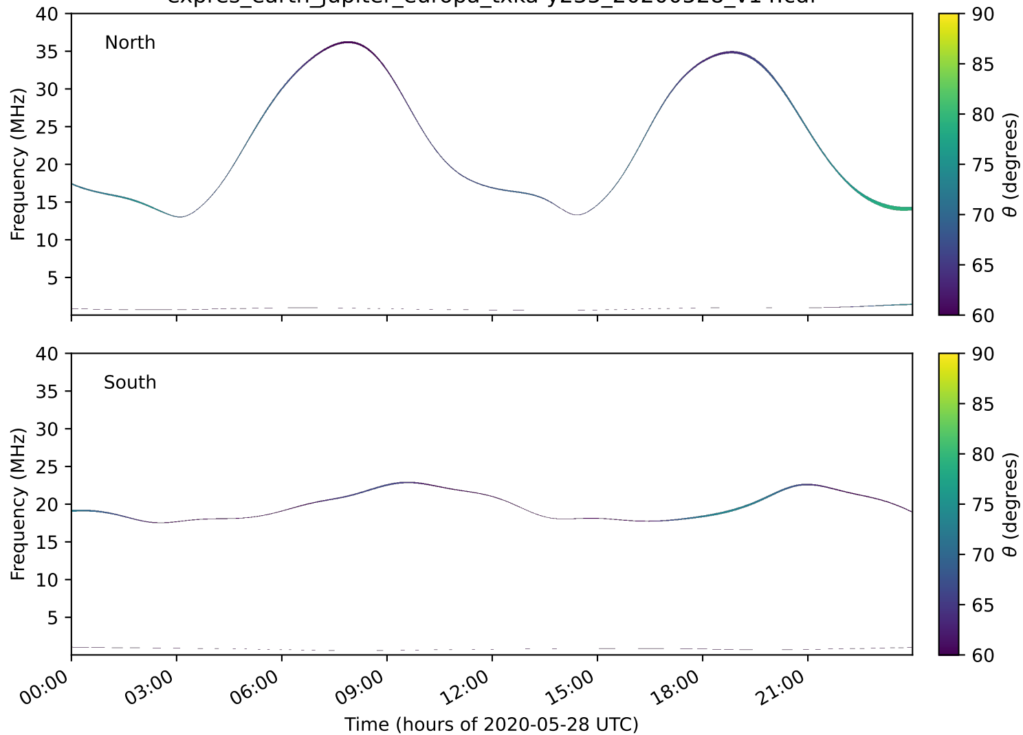
expres_earth_jupiter_europa_txka-y235_20200528_v14.cdf
