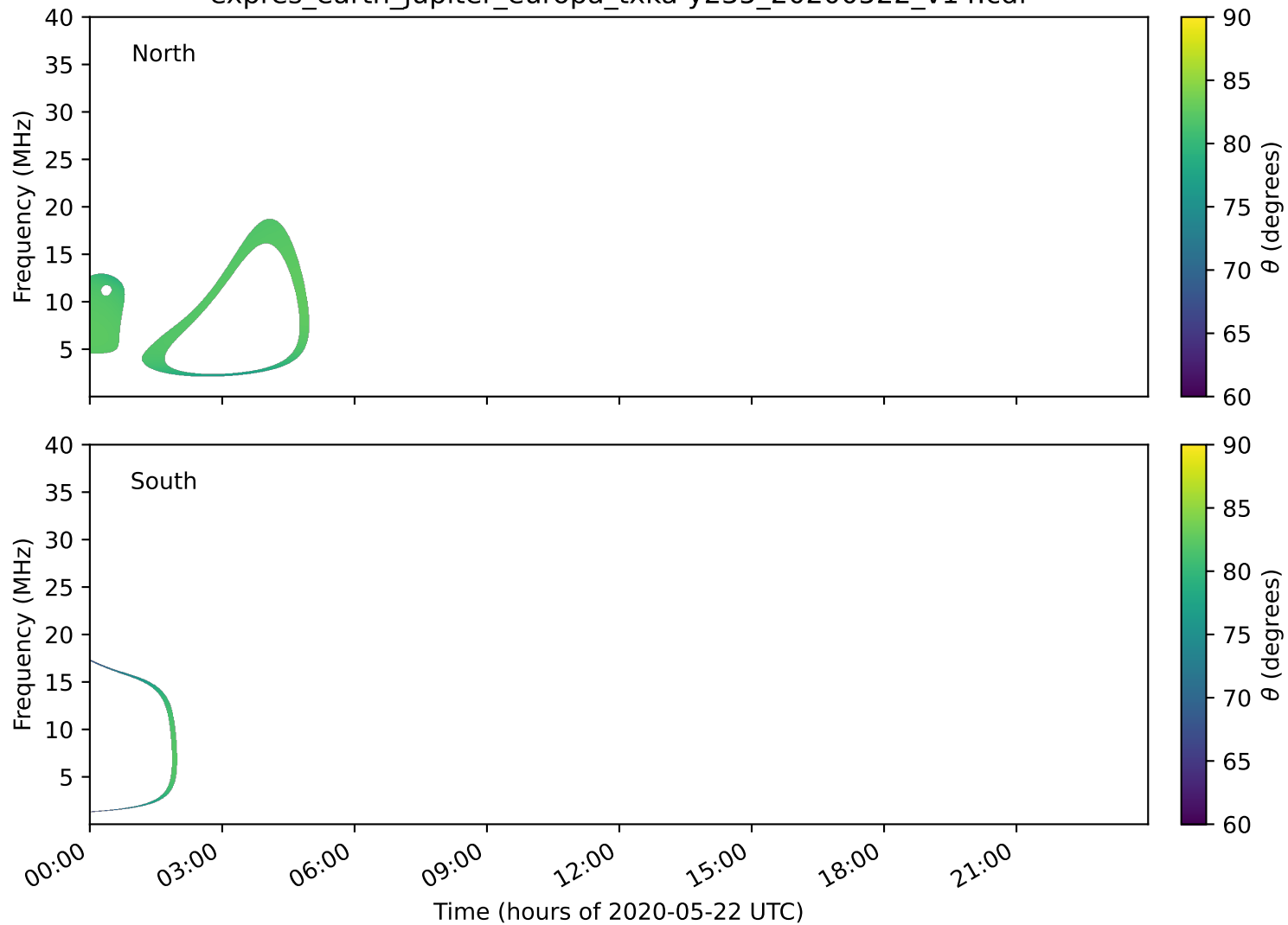
expres_earth_jupiter_europa_txka-y235_20200522_v14.cdf
