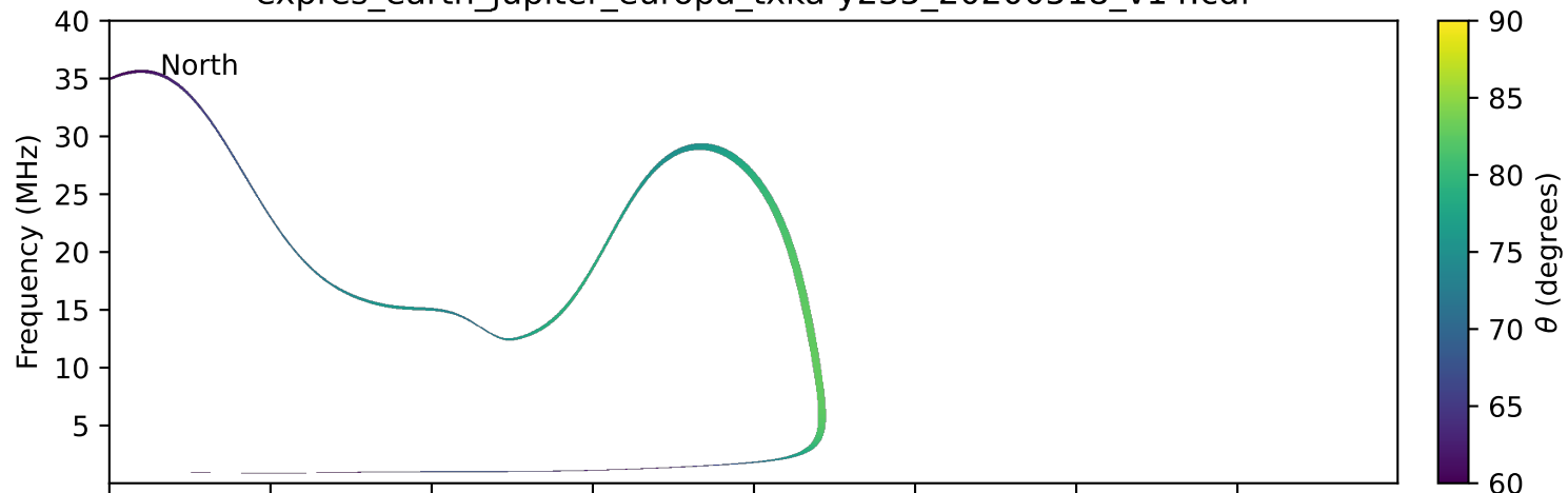
expres_earth_jupiter_europa_txka-y235_20200518_v14.cdf
