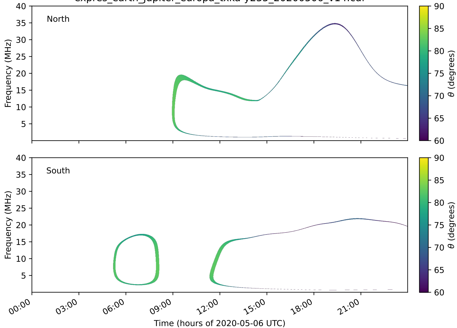
expres_earth_jupiter_europa_txka-y235_20200506_v14.cdf
