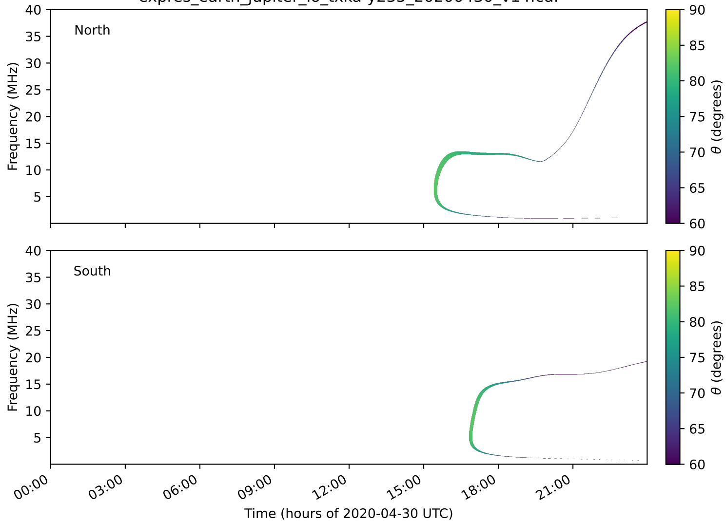
expres_earth_jupiter_io_txka-y235_20200430_v14.cdf
