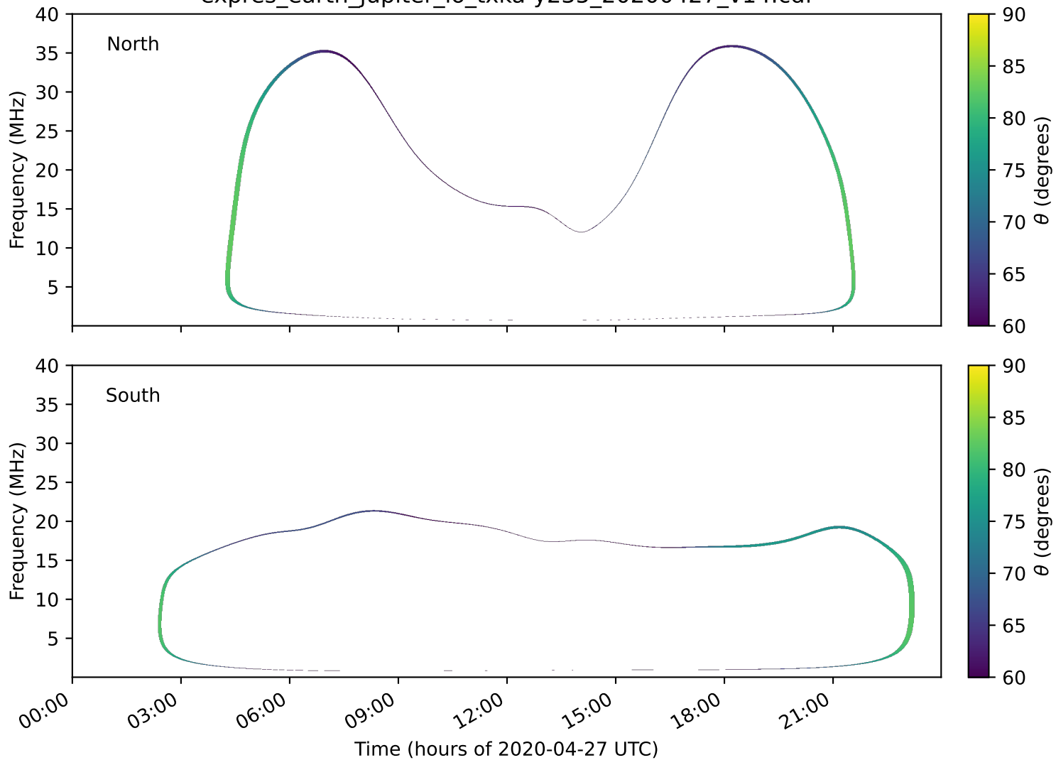
expres_earth_jupiter_io_txka-y235_20200427_v14.cdf
