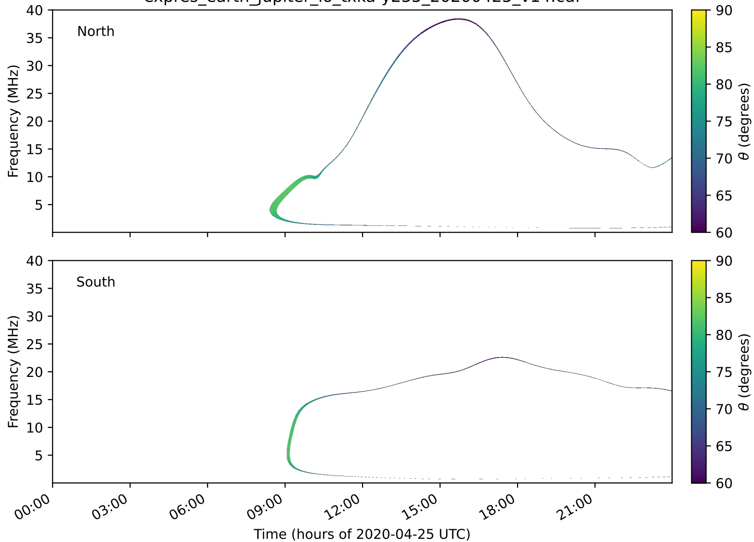
expres_earth_jupiter_io_txka-y235_20200425_v14.cdf
