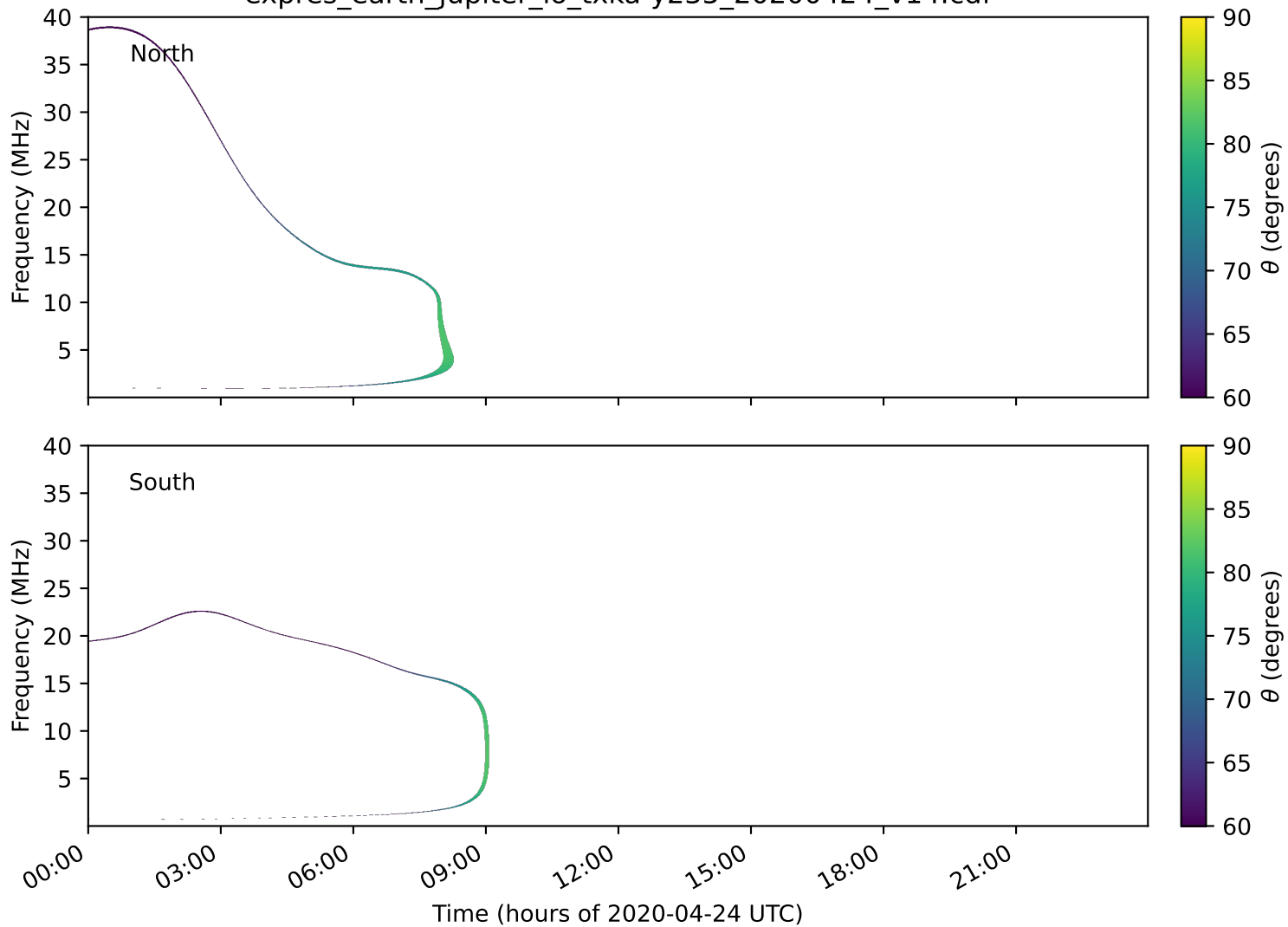
expres_earth_jupiter_io_txka-y235_20200424_v14.cdf
