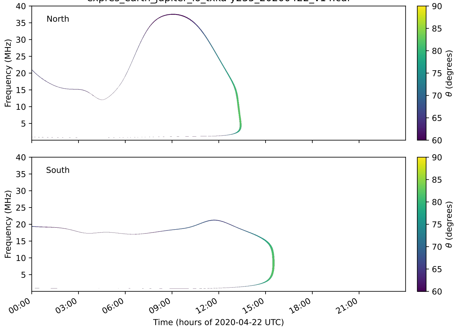
expres_earth_jupiter_io_txka-y235_20200422_v14.cdf
