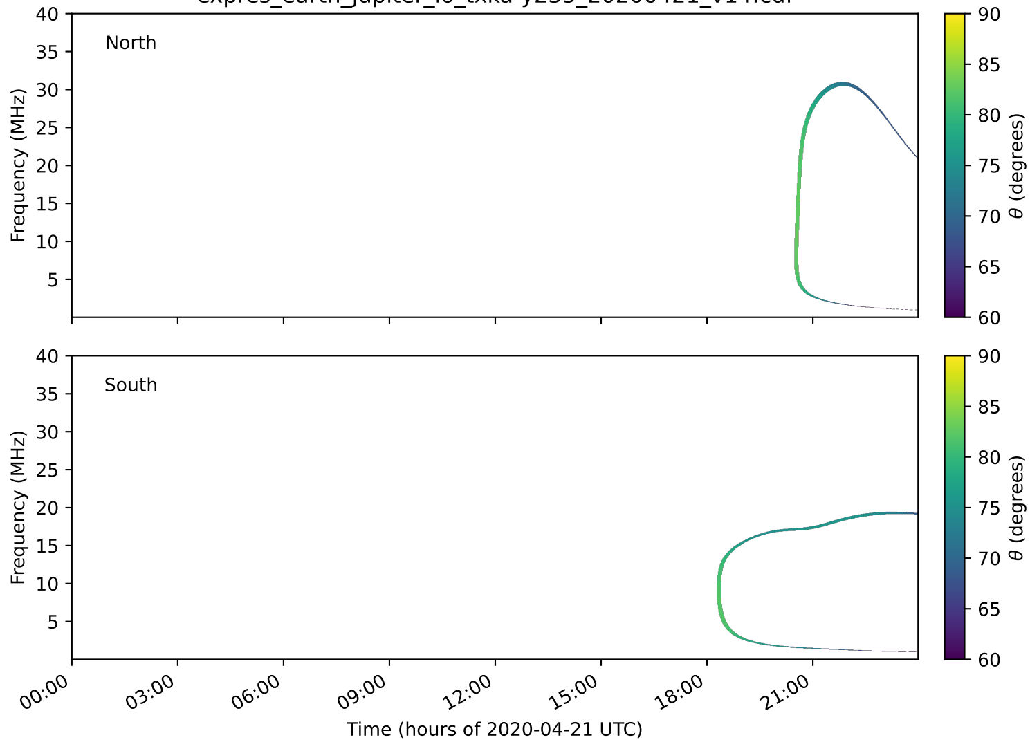
expres_earth_jupiter_io_txka-y235_20200421_v14.cdf
