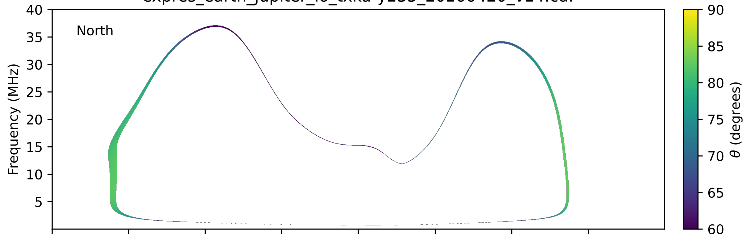
expres_earth_jupiter_io_txka-y235_20200420_v14.cdf
