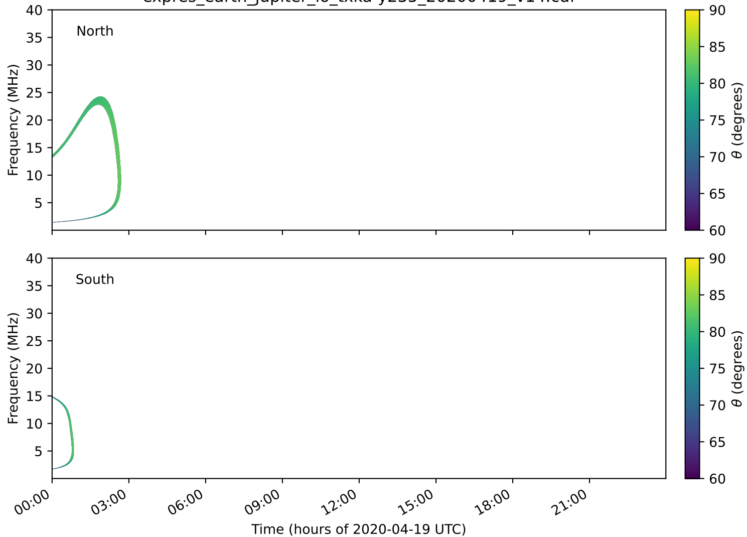
expres_earth_jupiter_io_txka-y235_20200419_v14.cdf
