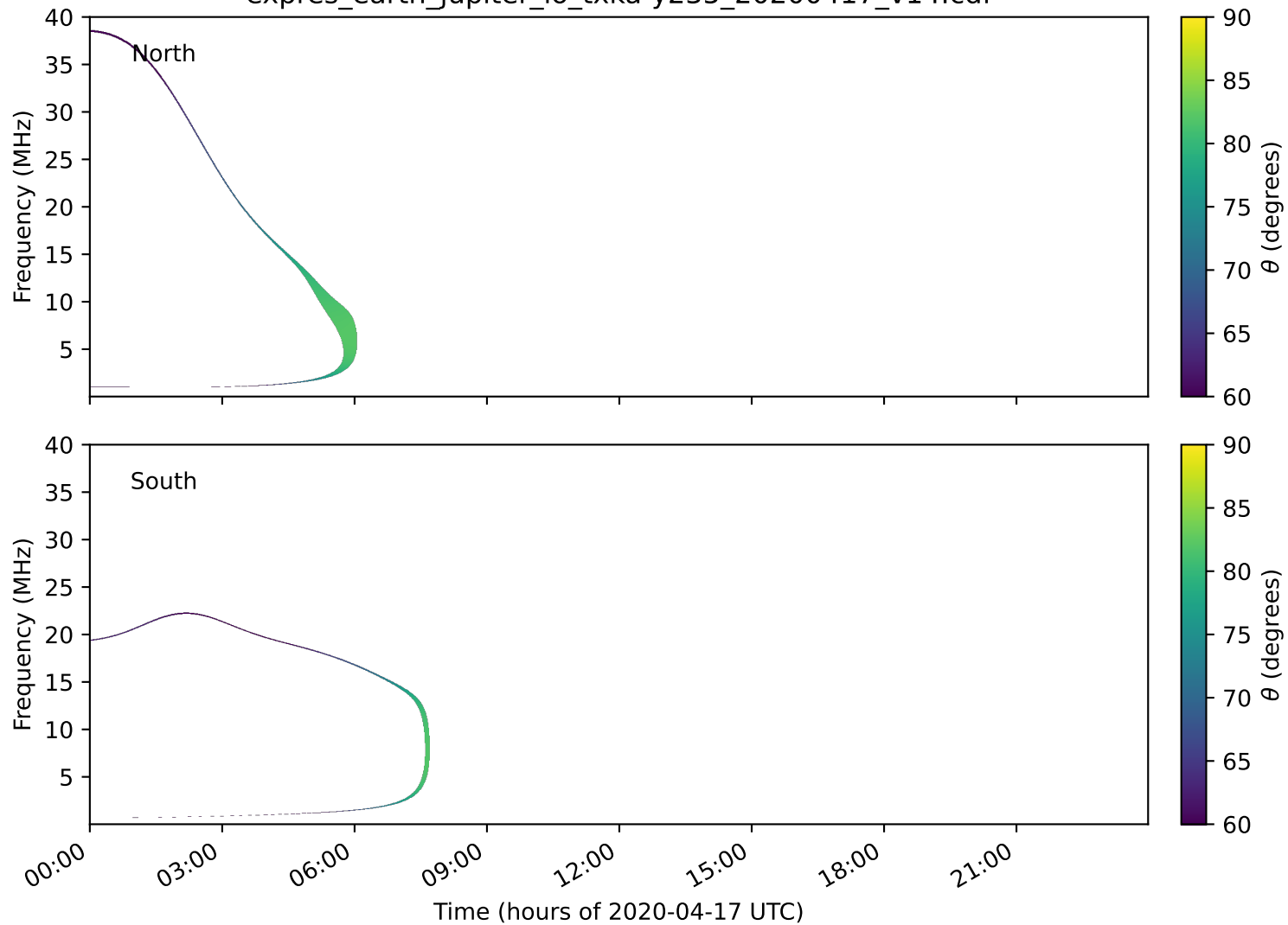
expres_earth_jupiter_io_txka-y235_20200417_v14.cdf
