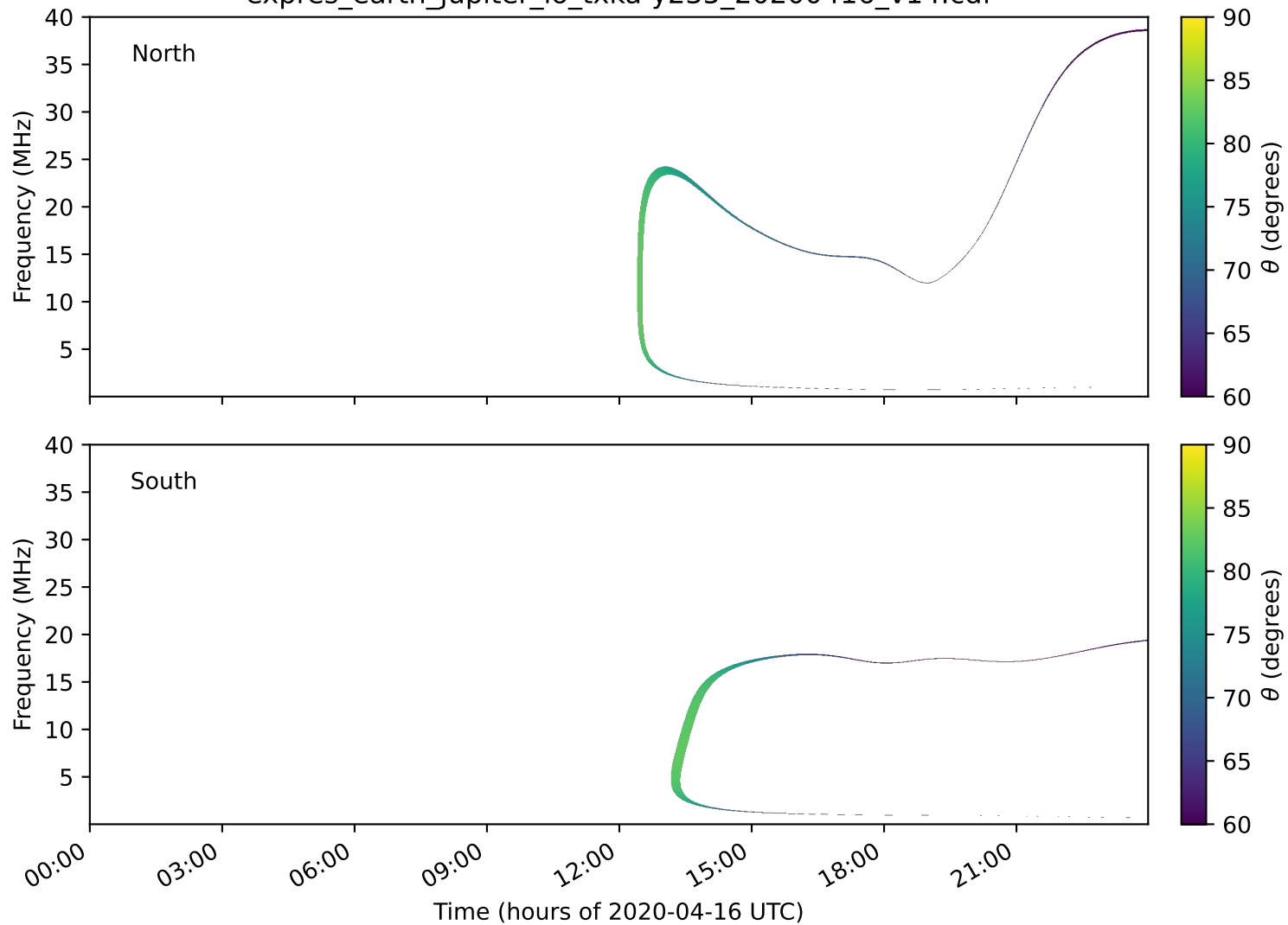
expres_earth_jupiter_io_txka-y235_20200416_v14.cdf
