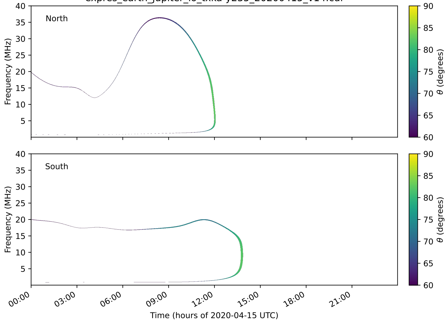
expres_earth_jupiter_io_txka-y235_20200415_v14.cdf
