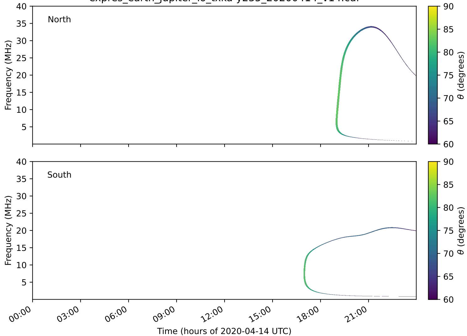
expres_earth_jupiter_io_txka-y235_20200414_v14.cdf
