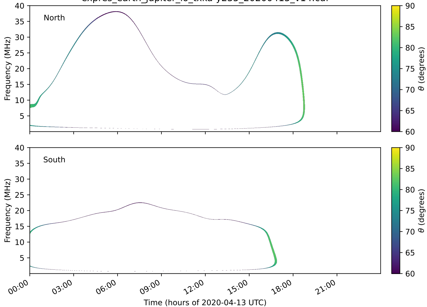
expres_earth_jupiter_io_txka-y235_20200413_v14.cdf
