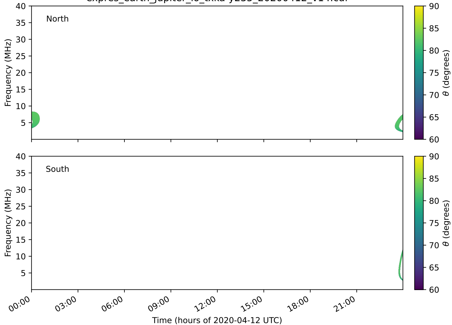
expres_earth_jupiter_io_txka-y235_20200412_v14.cdf
