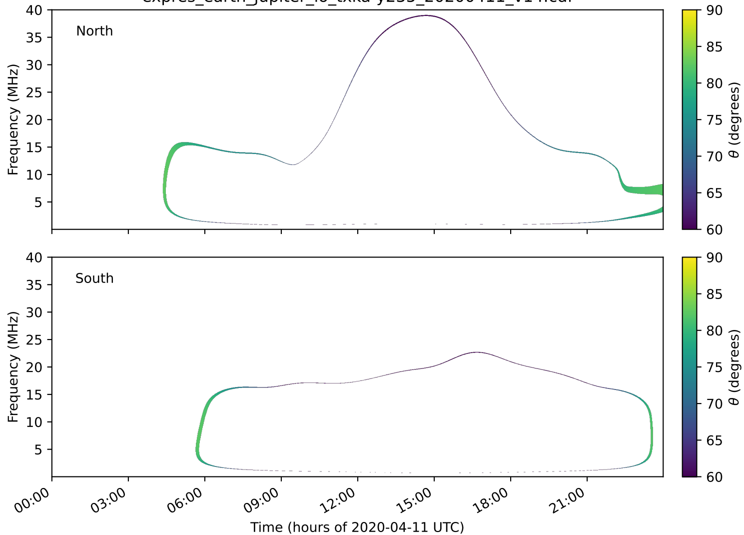
expres_earth_jupiter_io_txka-y235_20200411_v14.cdf
