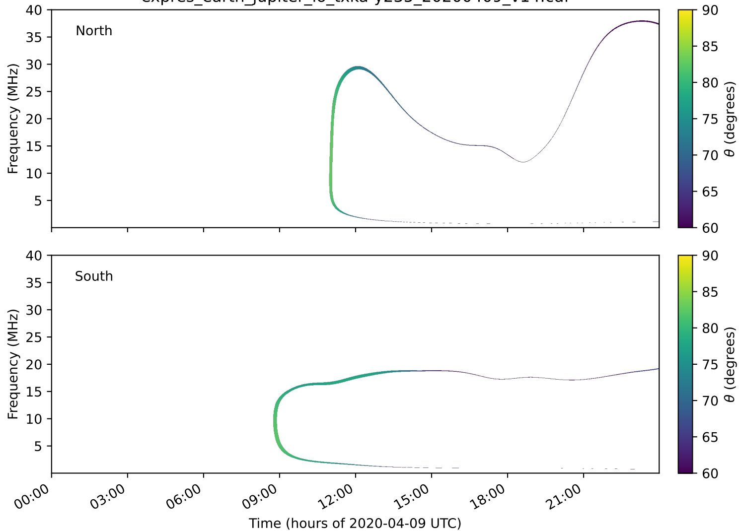
expres_earth_jupiter_io_txka-y235_20200409_v14.cdf
