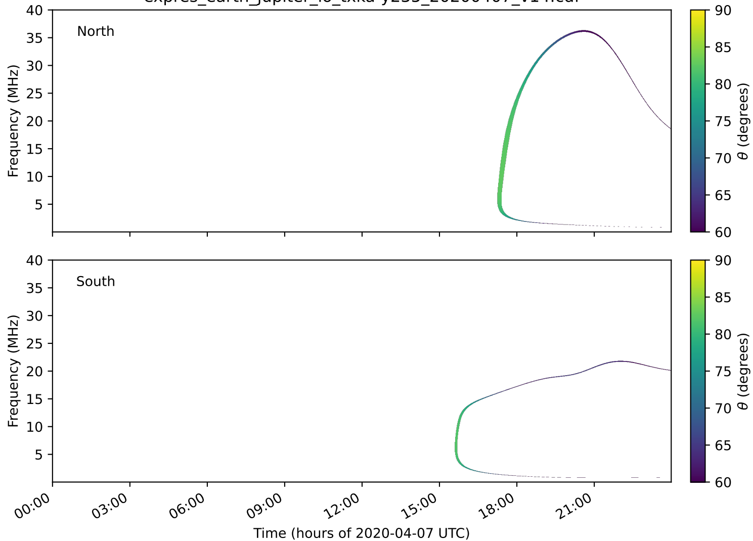
expres_earth_jupiter_io_txka-y235_20200407_v14.cdf
