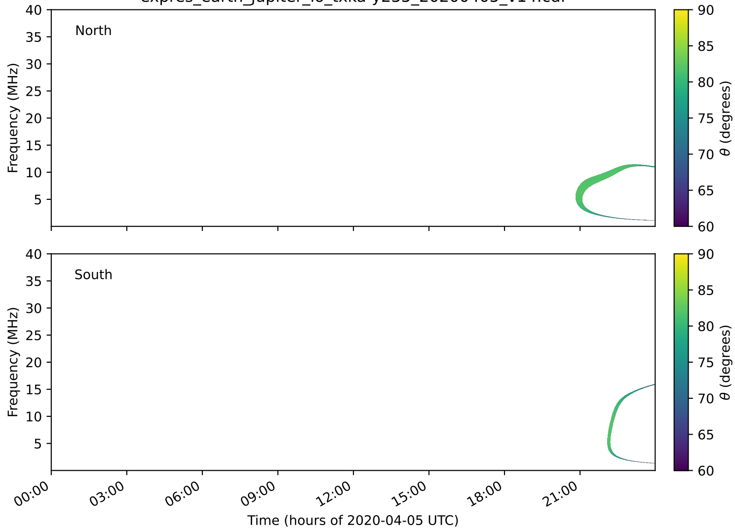
expres_earth_jupiter_io_txka-y235_20200405_v14.cdf
