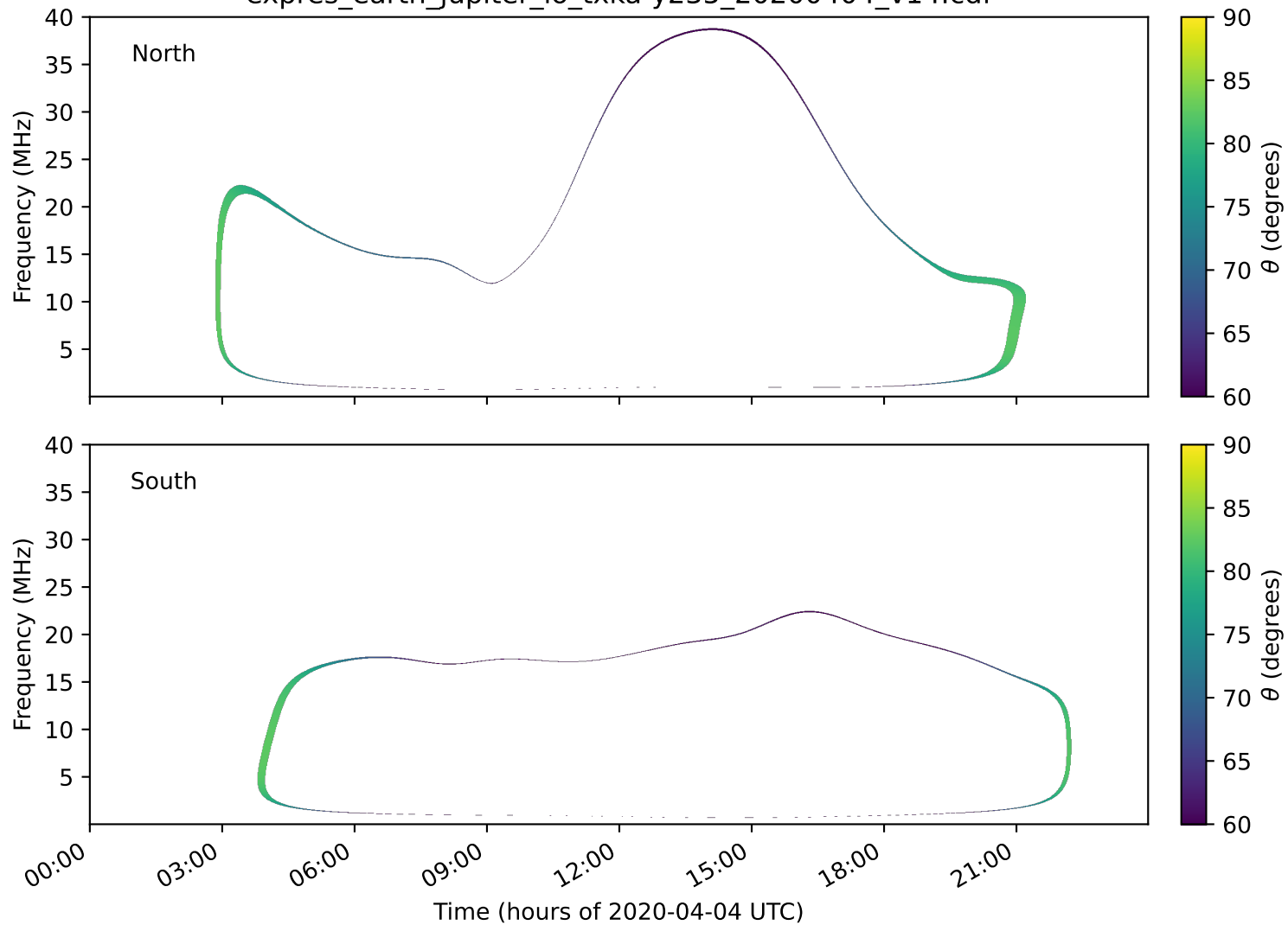
expres_earth_jupiter_io_txka-y235_20200404_v14.cdf
