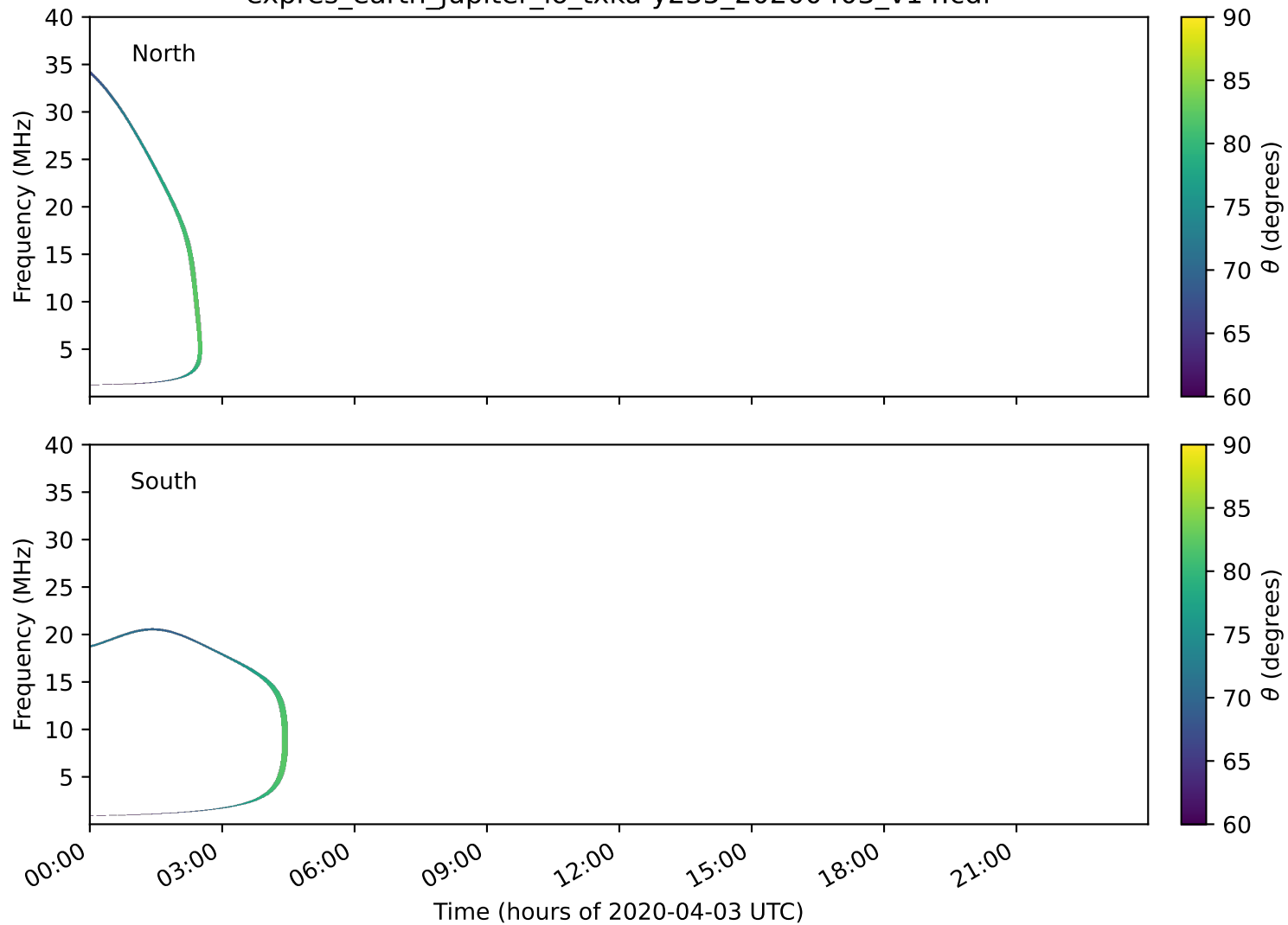
expres_earth_jupiter_io_txka-y235_20200403_v14.cdf
