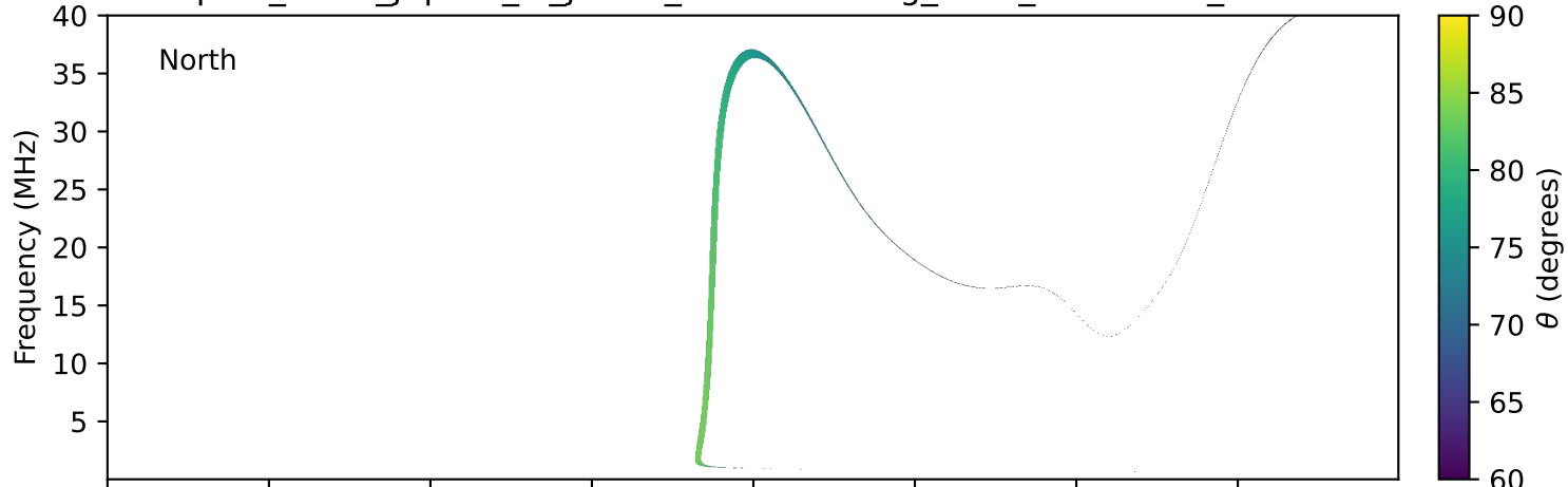
expres_earth_jupiter_io_jrm33_lossc-wid1deg_3kev_20200409_v11.cdf
