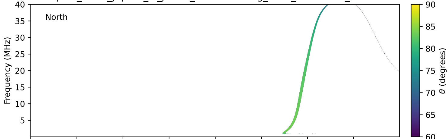
expres_earth_jupiter_io_jrm33_lossc-wid1deg_3kev_20200407_v11.cdf
