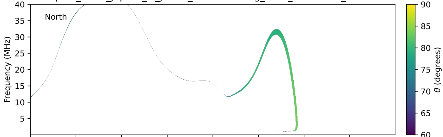
expres_earth_jupiter_io_jrm33_lossc-wid1deg_3kev_20200406_v11.cdf
