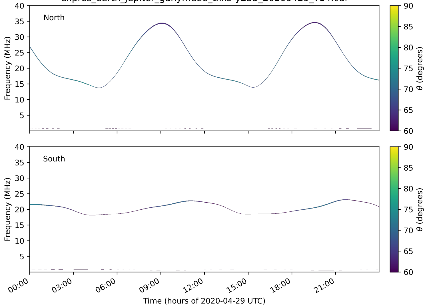
expres_earth_jupiter_ganymede_txka-y235_20200429_v14.cdf
