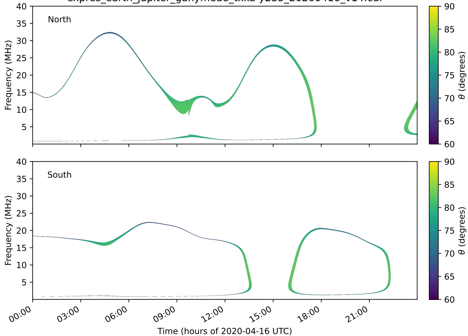
expres_earth_jupiter_ganymede_txka-y235_20200416_v14.cdf
