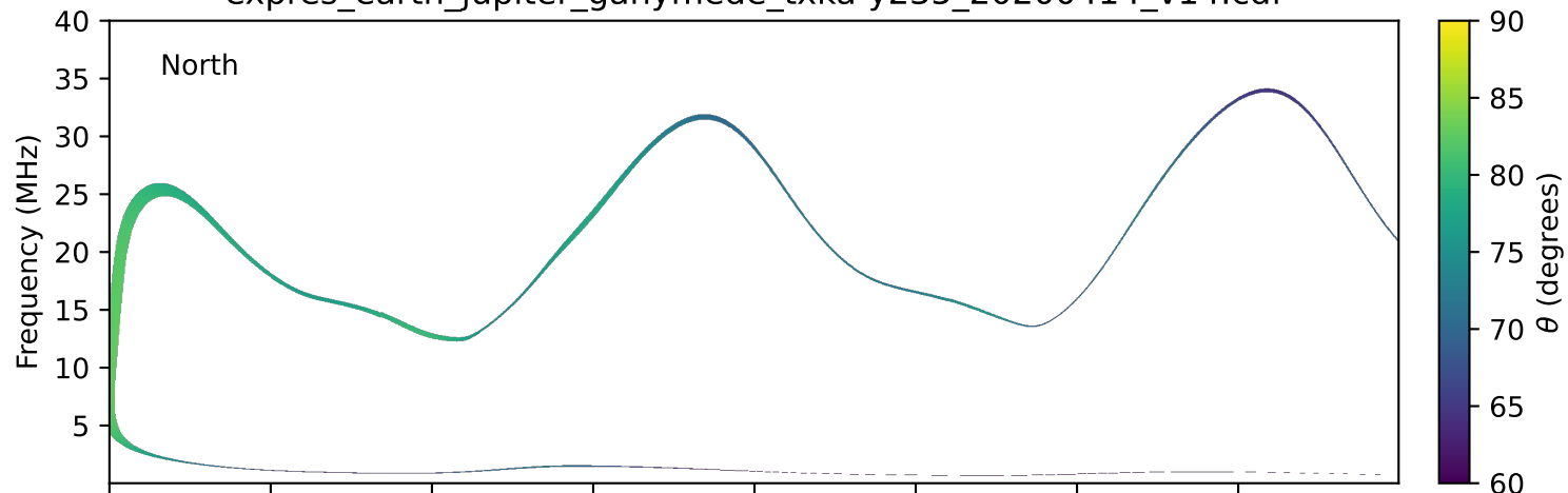
expres_earth_jupiter_ganymede_txka-y235_20200414_v14.cdf
