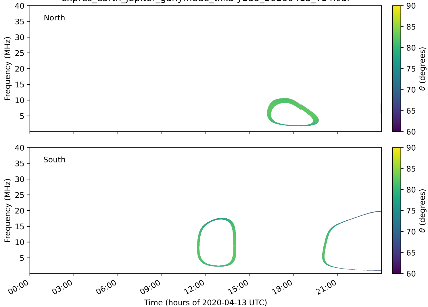
expres_earth_jupiter_ganymede_txka-y235_20200413_v14.cdf
