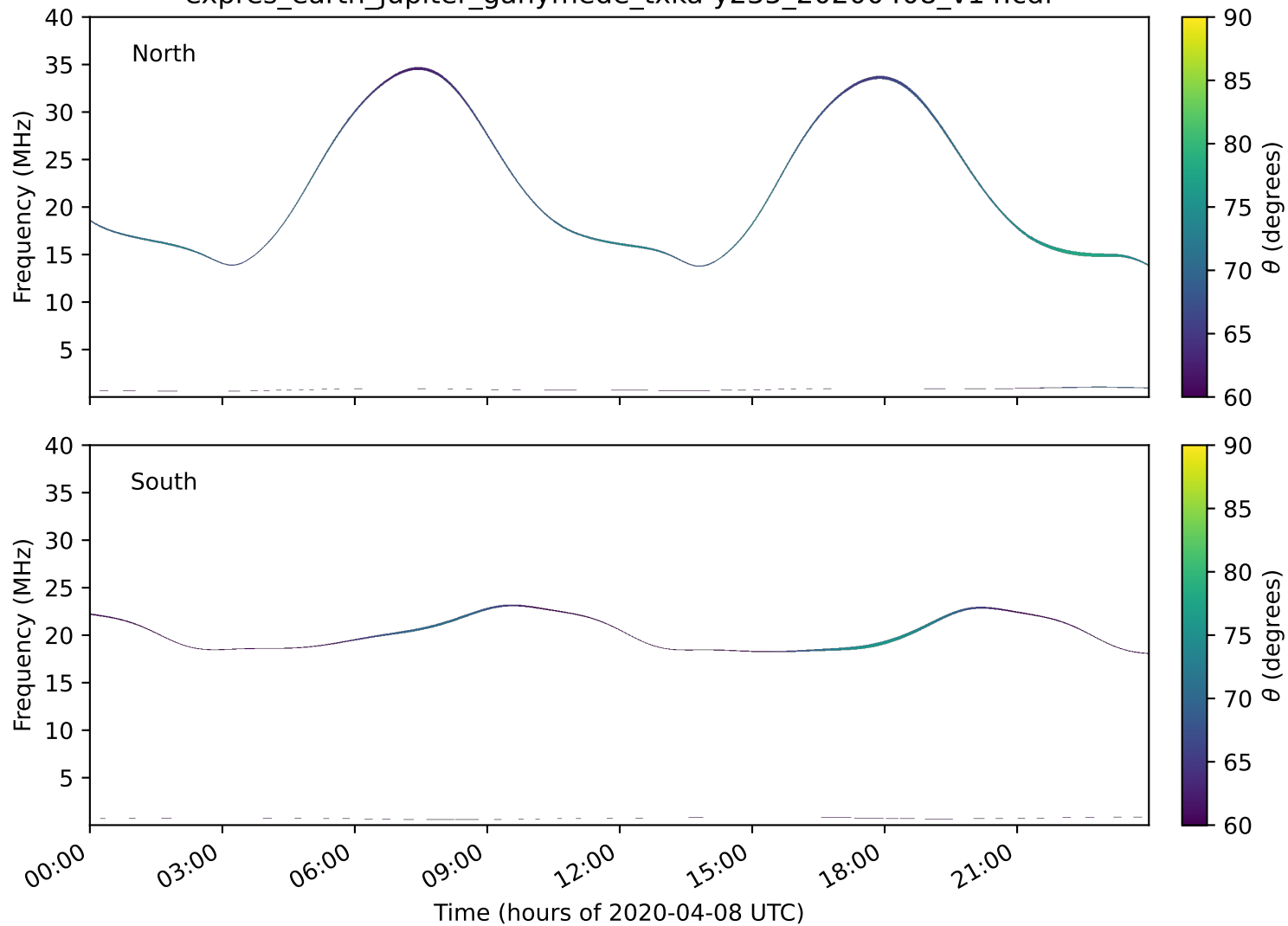
expres_earth_jupiter_ganymede_txka-y235_20200408_v14.cdf
