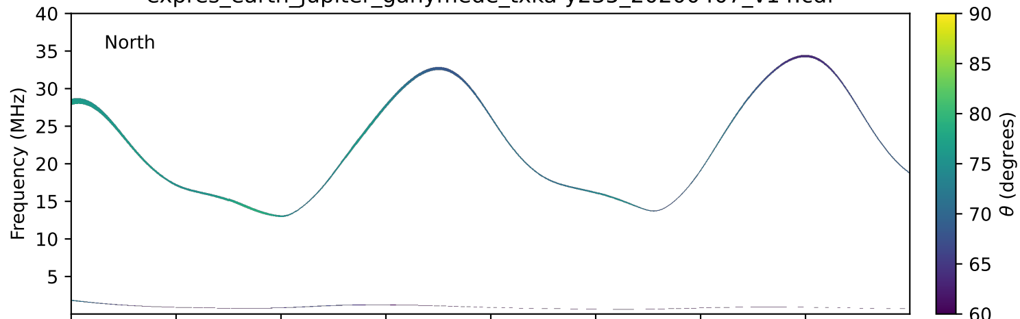
expres_earth_jupiter_ganymede_txka-y235_20200407_v14.cdf
