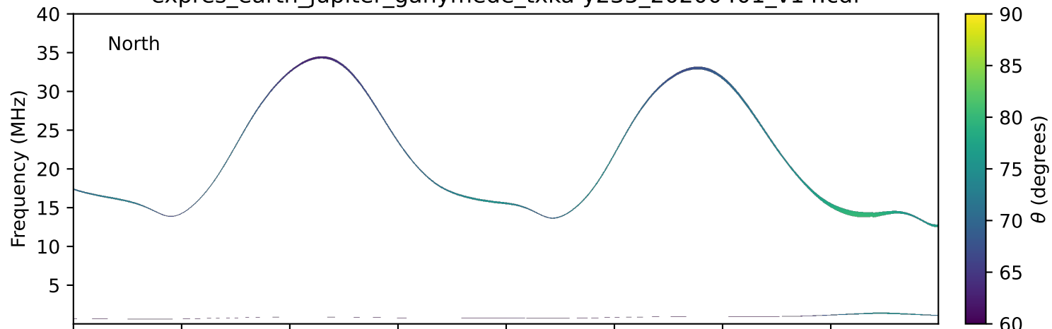
expres_earth_jupiter_ganymede_txka-y235_20200401_v14.cdf
