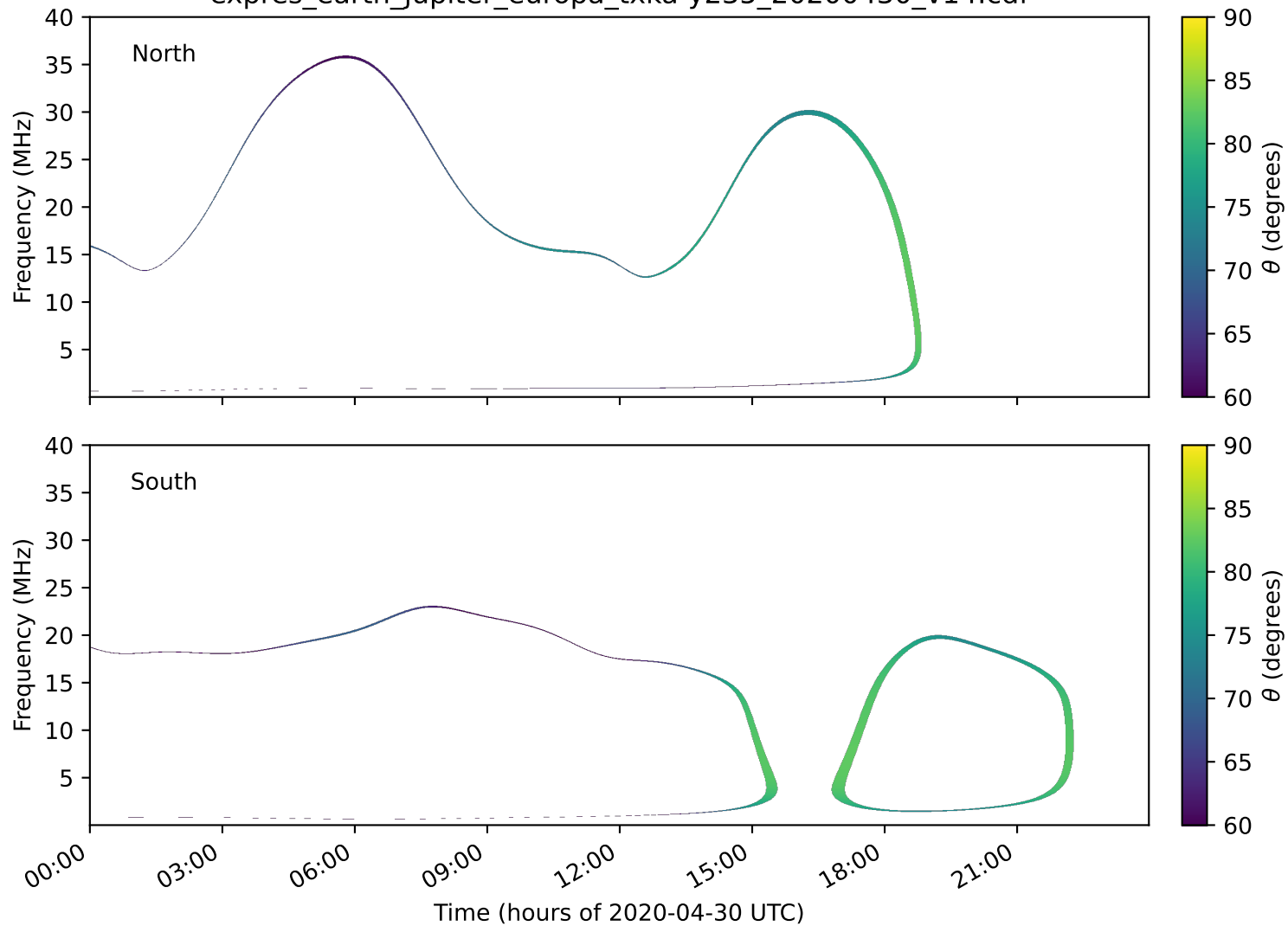
expres_earth_jupiter_europa_txka-y235_20200430_v14.cdf
