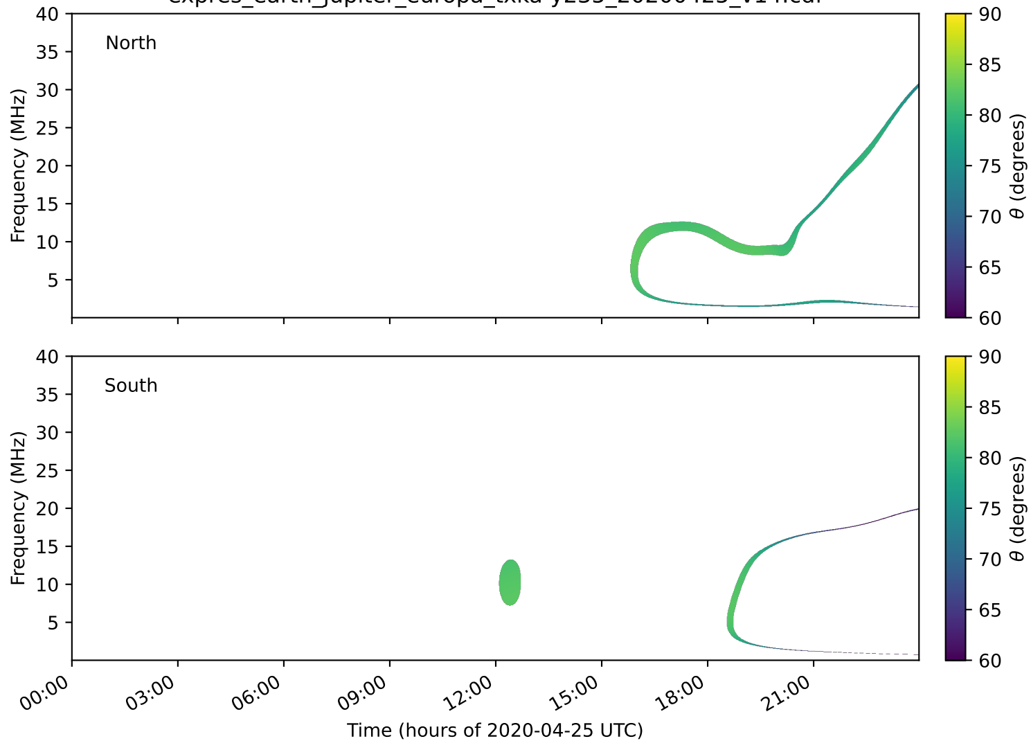
expres_earth_jupiter_europa_txka-y235_20200425_v14.cdf
