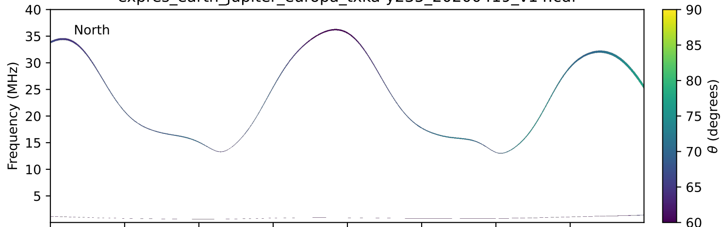
expres_earth_jupiter_europa_txka-y235_20200419_v14.cdf
