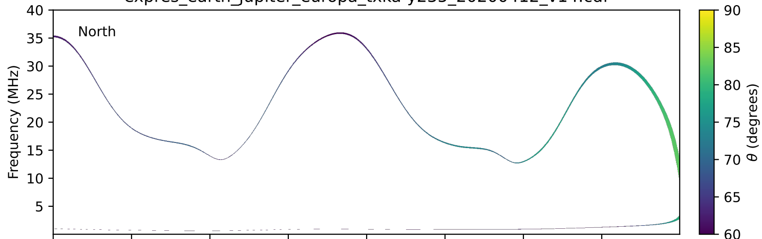
expres_earth_jupiter_europa_txka-y235_20200412_v14.cdf
