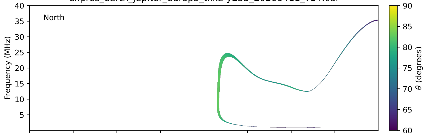
expres_earth_jupiter_europa_txka-y235_20200411_v14.cdf
