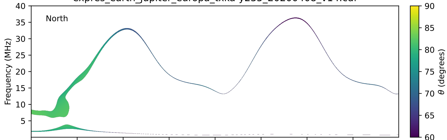
expres_earth_jupiter_europa_txka-y235_20200408_v14.cdf
