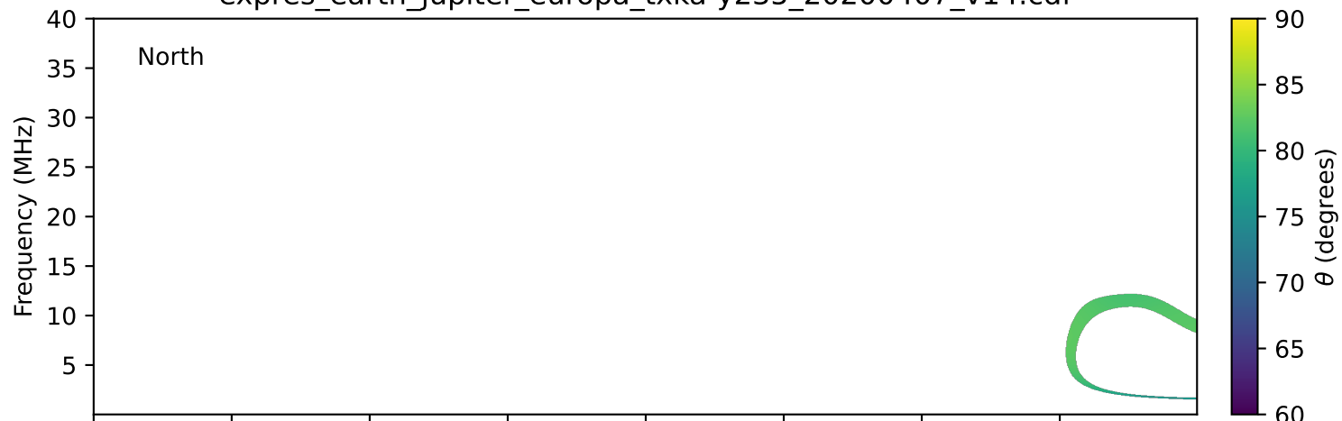
expres_earth_jupiter_europa_txka-y235_20200407_v14.cdf
