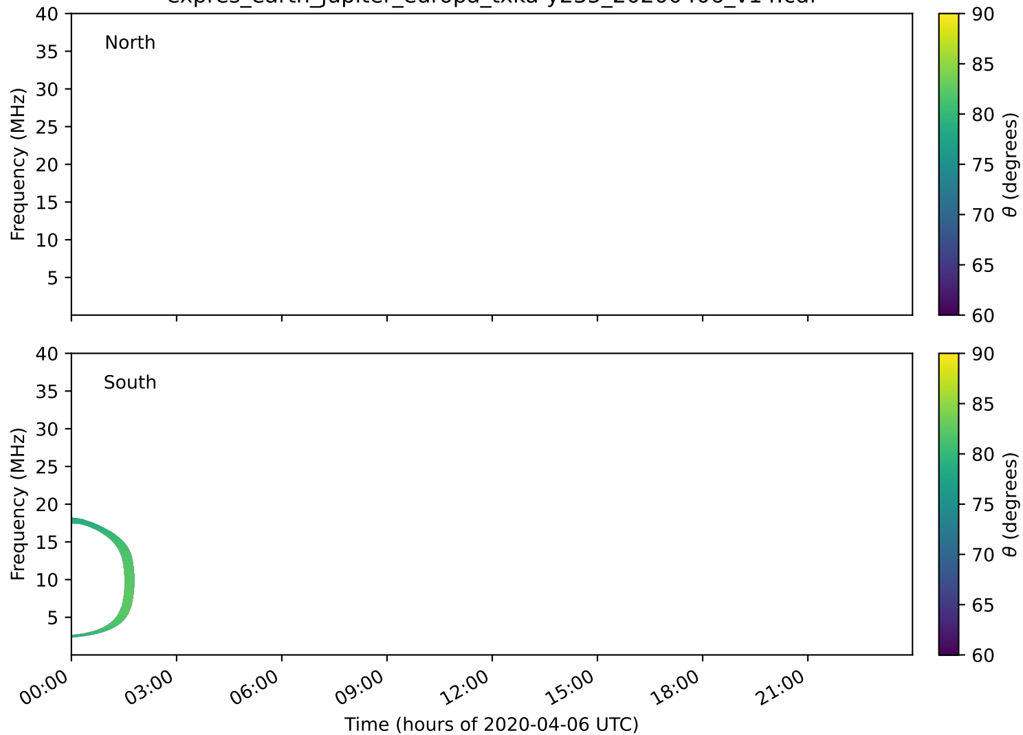
expres_earth_jupiter_europa_txka-y235_20200406_v14.cdf
