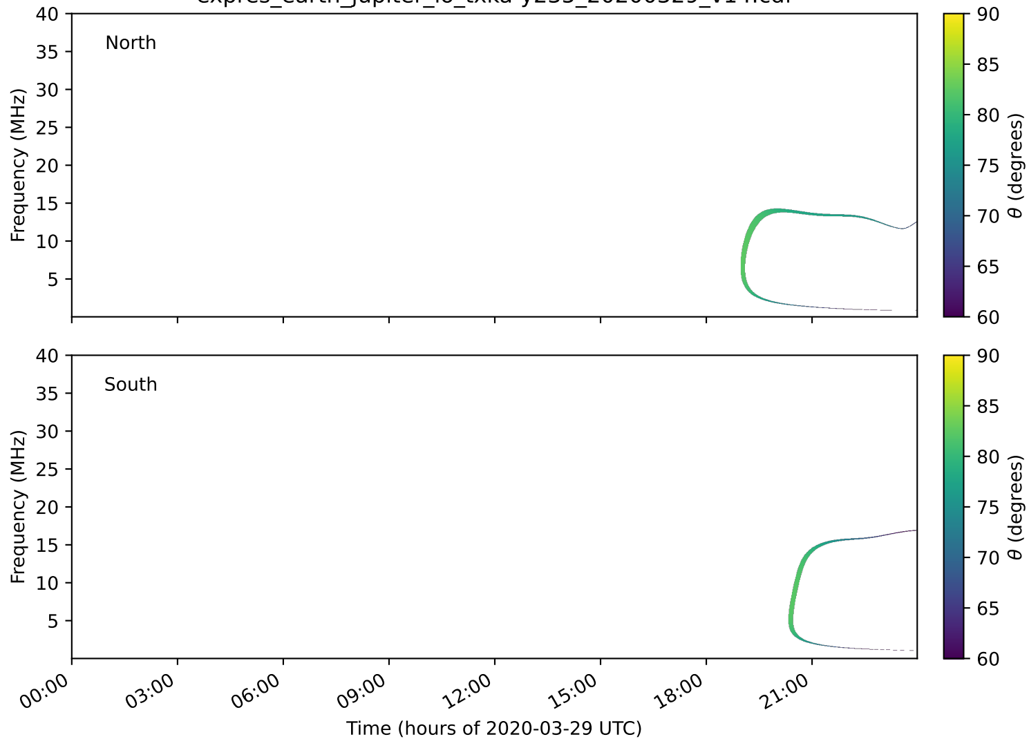
expres_earth_jupiter_io_txka-y235_20200329_v14.cdf
