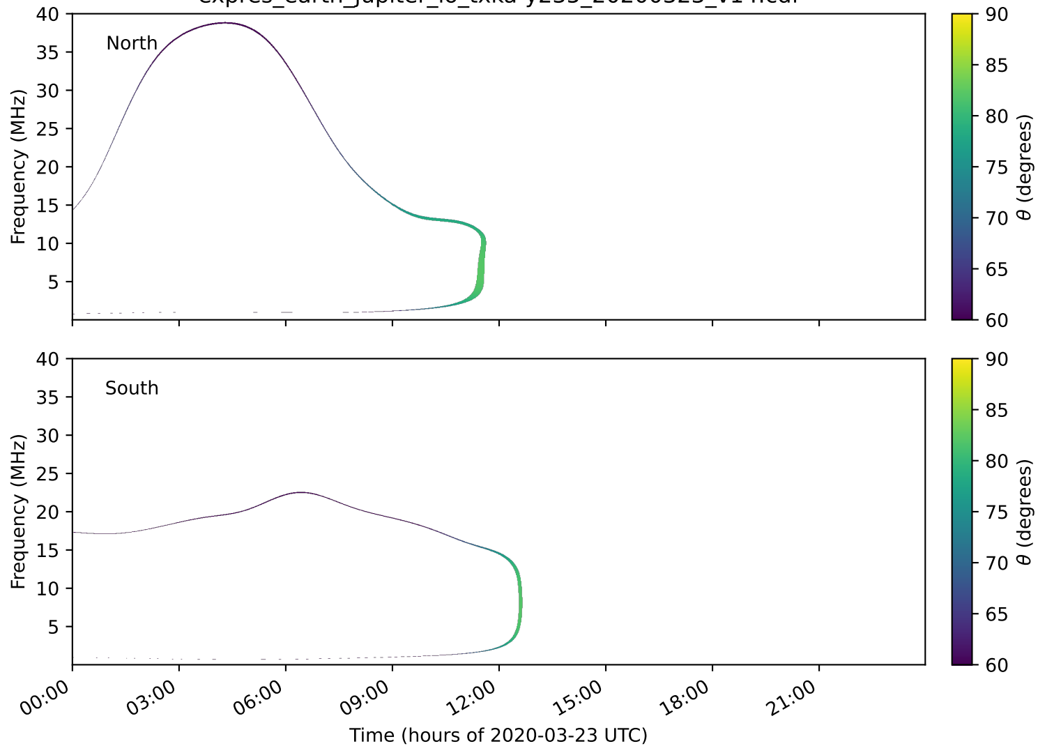
expres_earth_jupiter_io_txka-y235_20200323_v14.cdf
