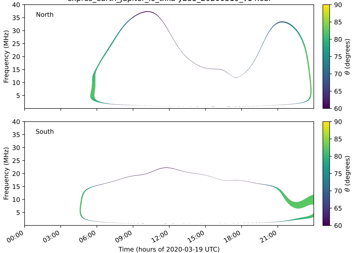
expres_earth_jupiter_io_txka-y235_20200319_v14.cdf
