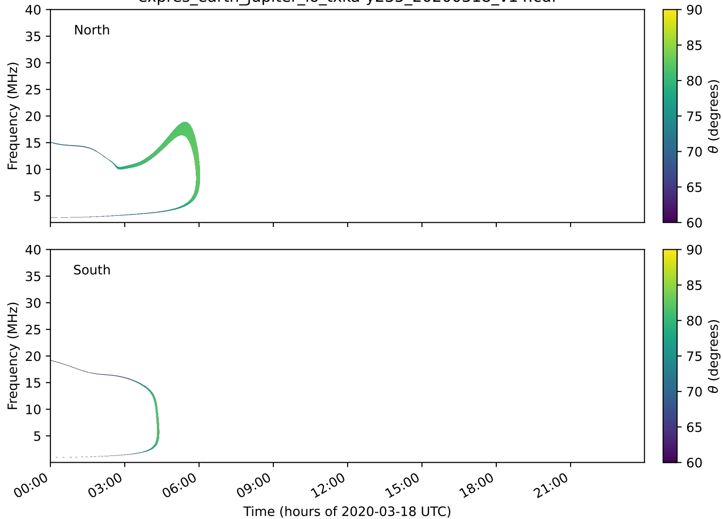
expres_earth_jupiter_io_txka-y235_20200318_v14.cdf
