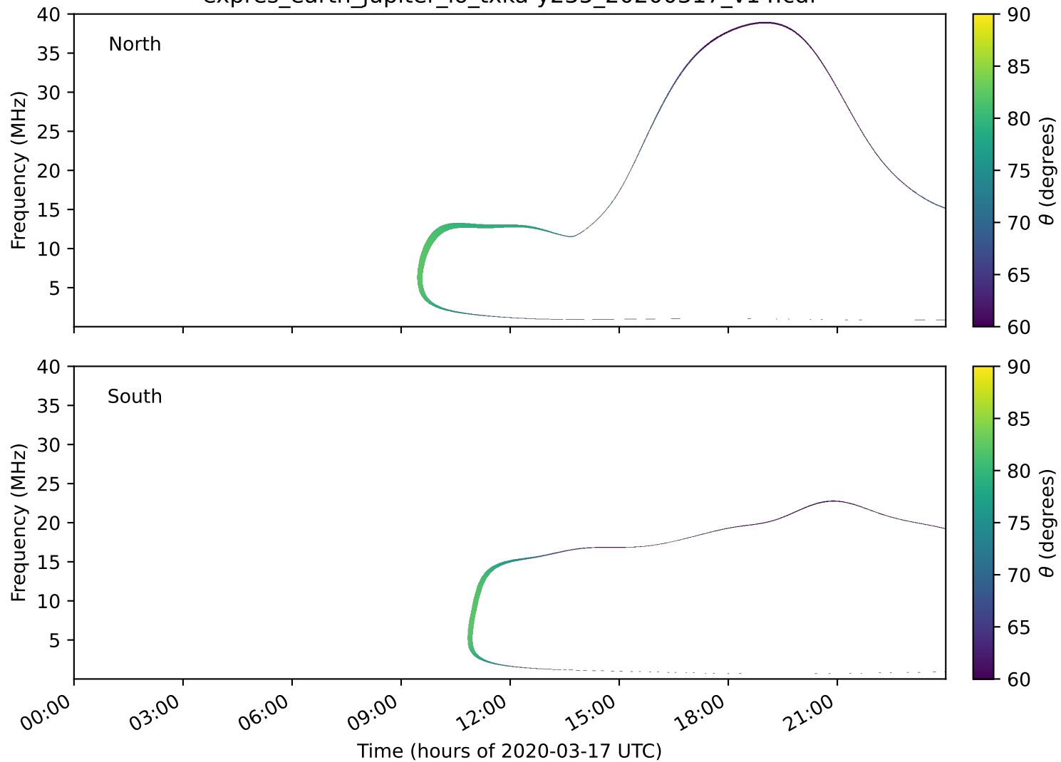
expres_earth_jupiter_io_txka-y235_20200317_v14.cdf
