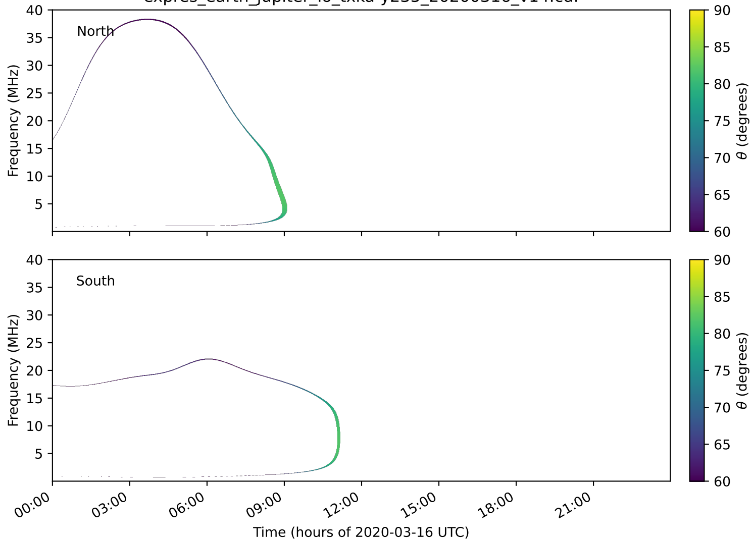
expres_earth_jupiter_io_txka-y235_20200316_v14.cdf
